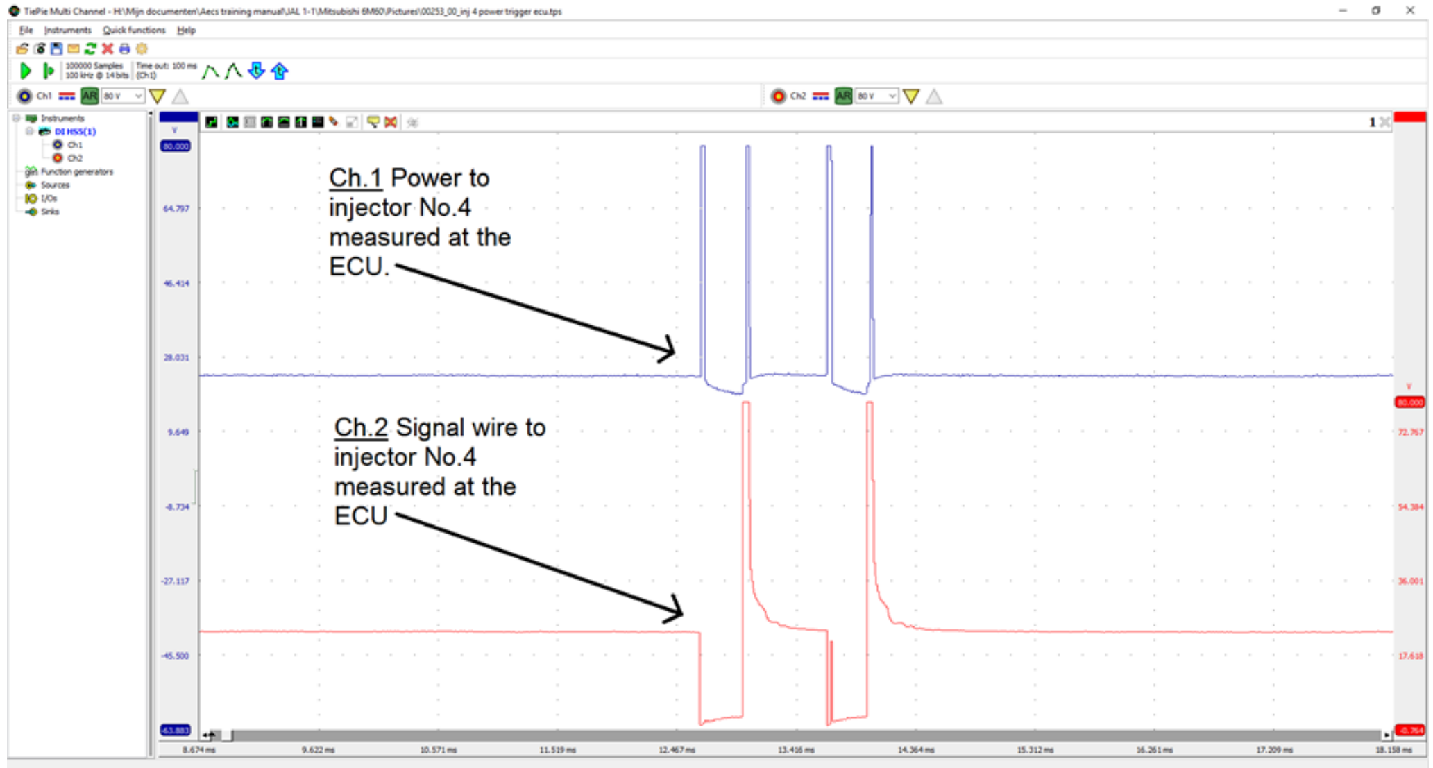
Picture 1: Both wires to the injector bank2 measured at the ECU.
