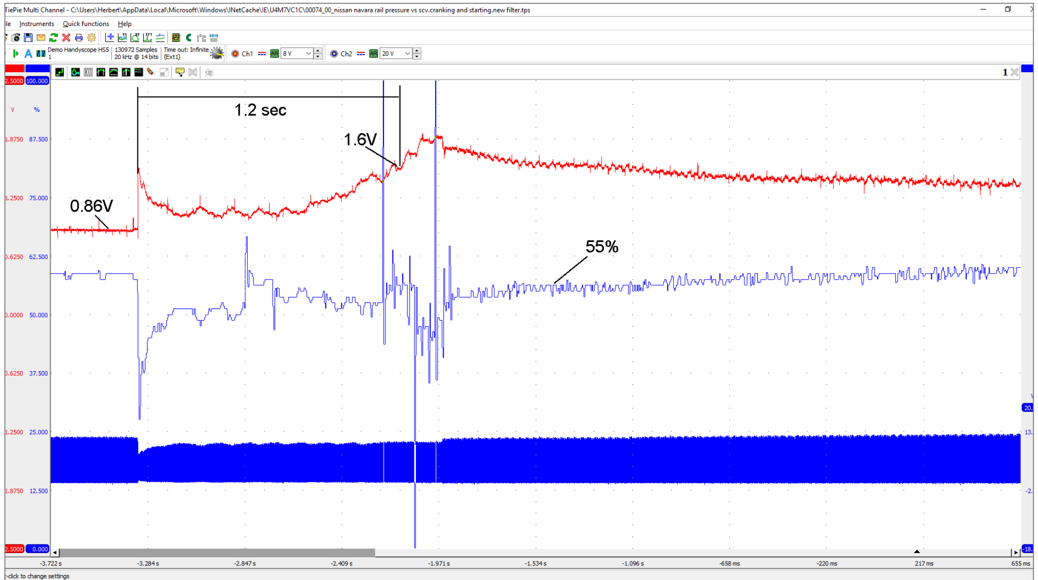
Picture 3: ATS scope recording of starting and firing up engine with the genuine filter fitted.
