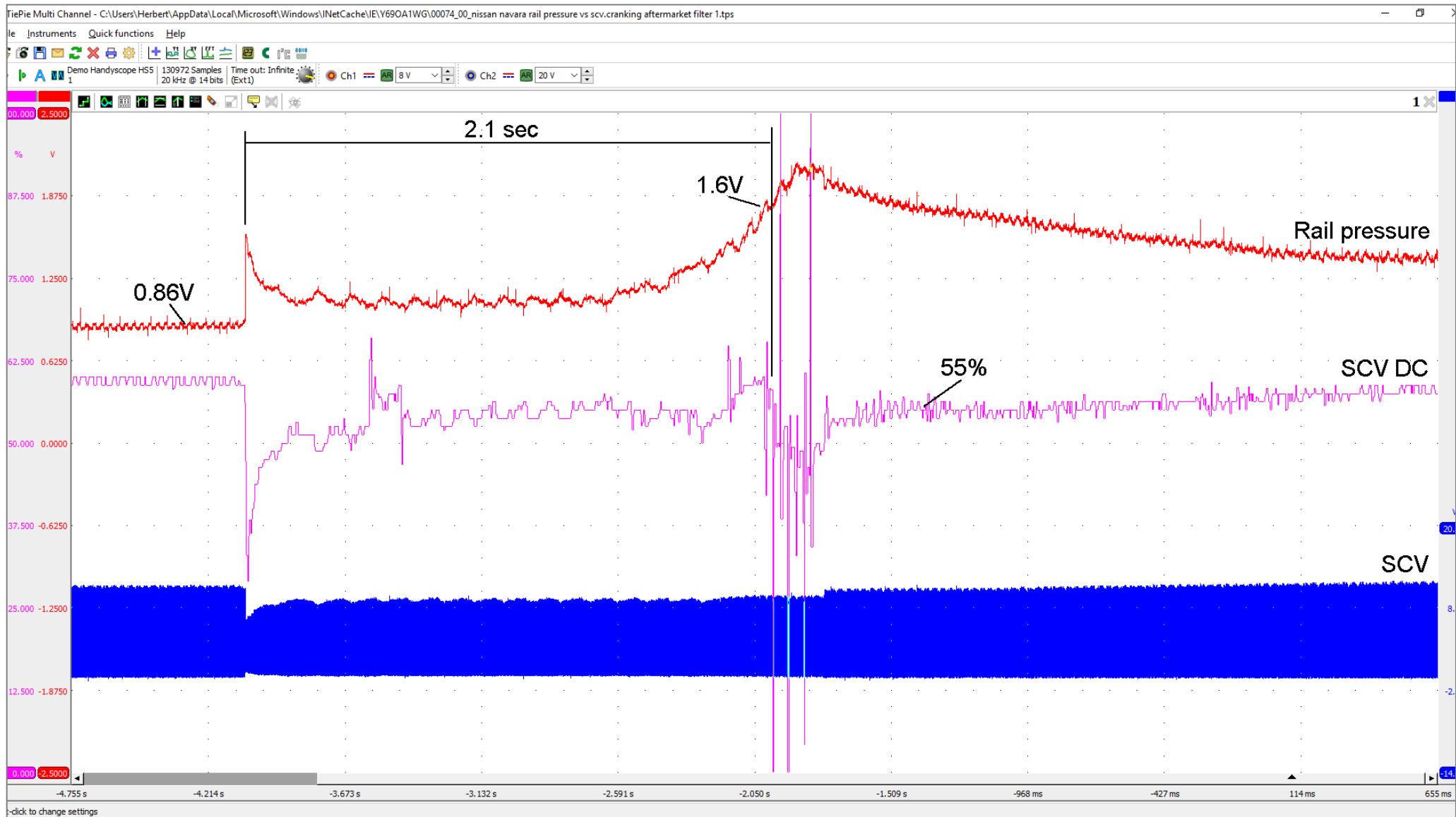
Picture 2: ATS scope recording of starting and firing up engine when the pump is drawing fuel through the filter.
