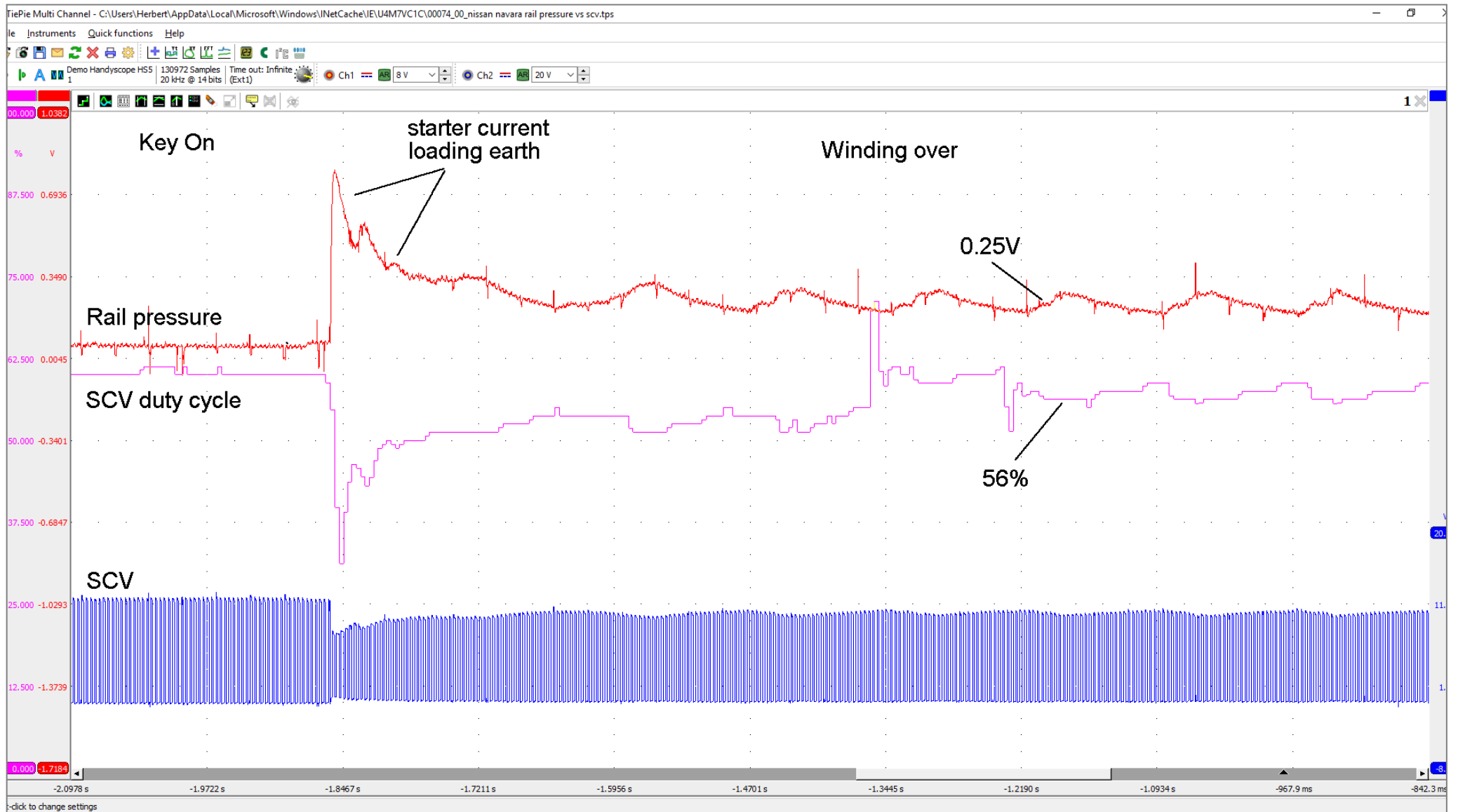
Picture 1 - ATS scope picture of Suction Control Valve (SCV) vs rail pressure
