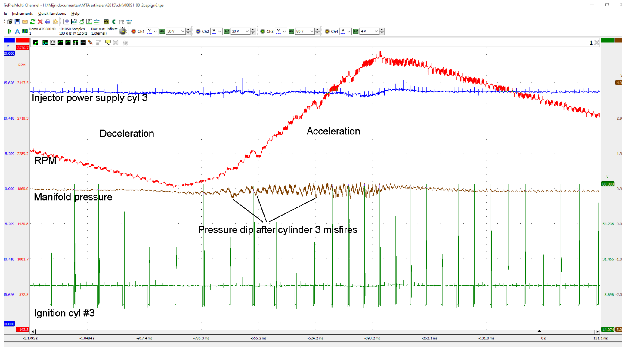
Picture 3: ATS scope recording of manifold pressure (with pressure sensor) during acceleration.
