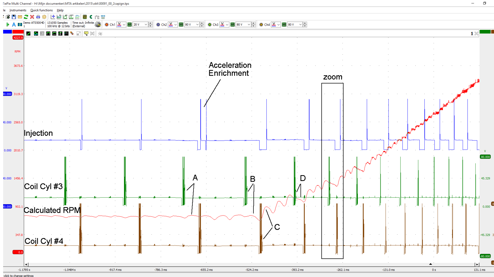
Picture 1: ATS 5004d recording of the crankshaft sensor, Injection and the coils on cylinder 3 and 4.
