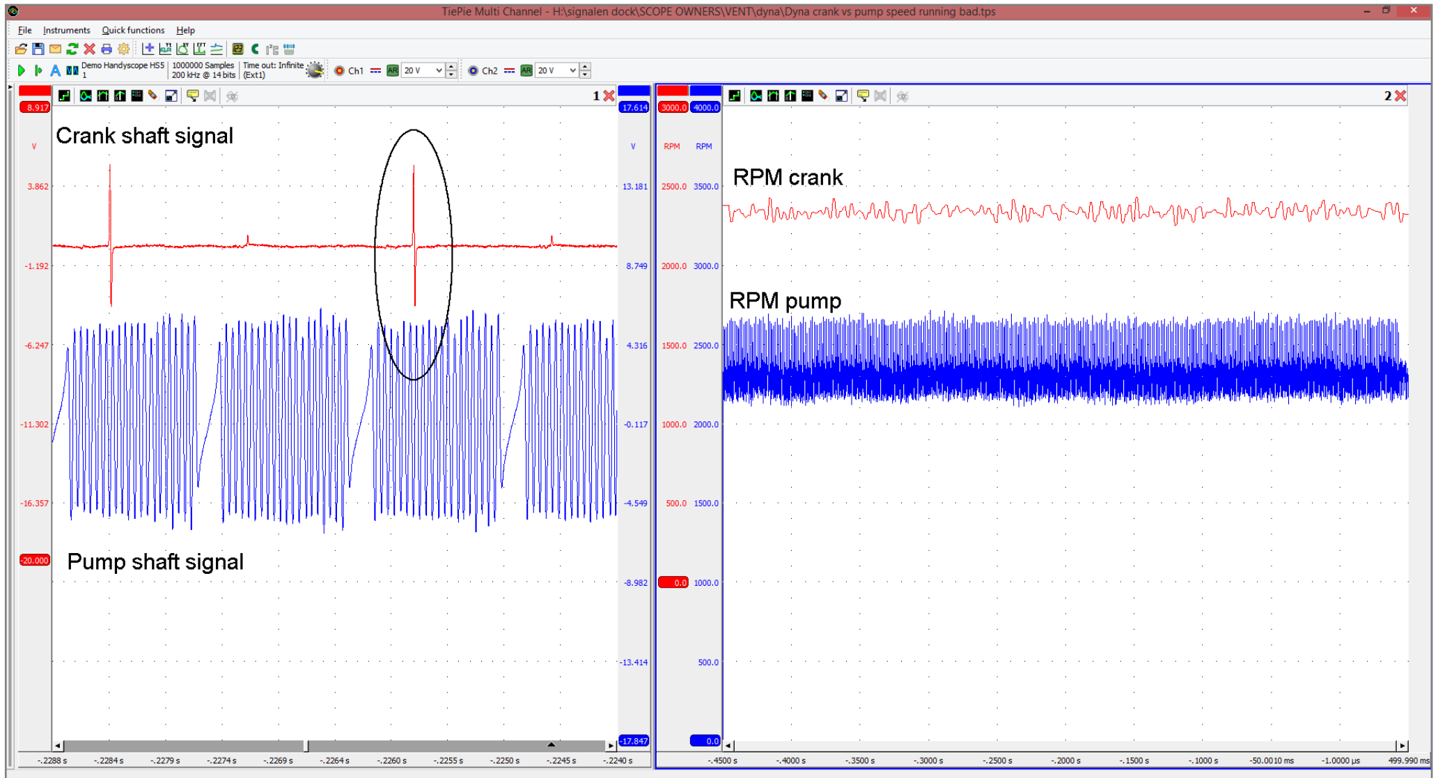
Picture 7: Split screen recording ATS 500XM of Pump shaft vs crank shaft sensor, when running bad.
