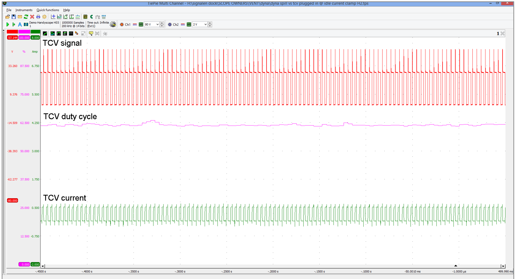
Picture 3: ATS scope recording of TCV voltage over current, running good (cold engine).
