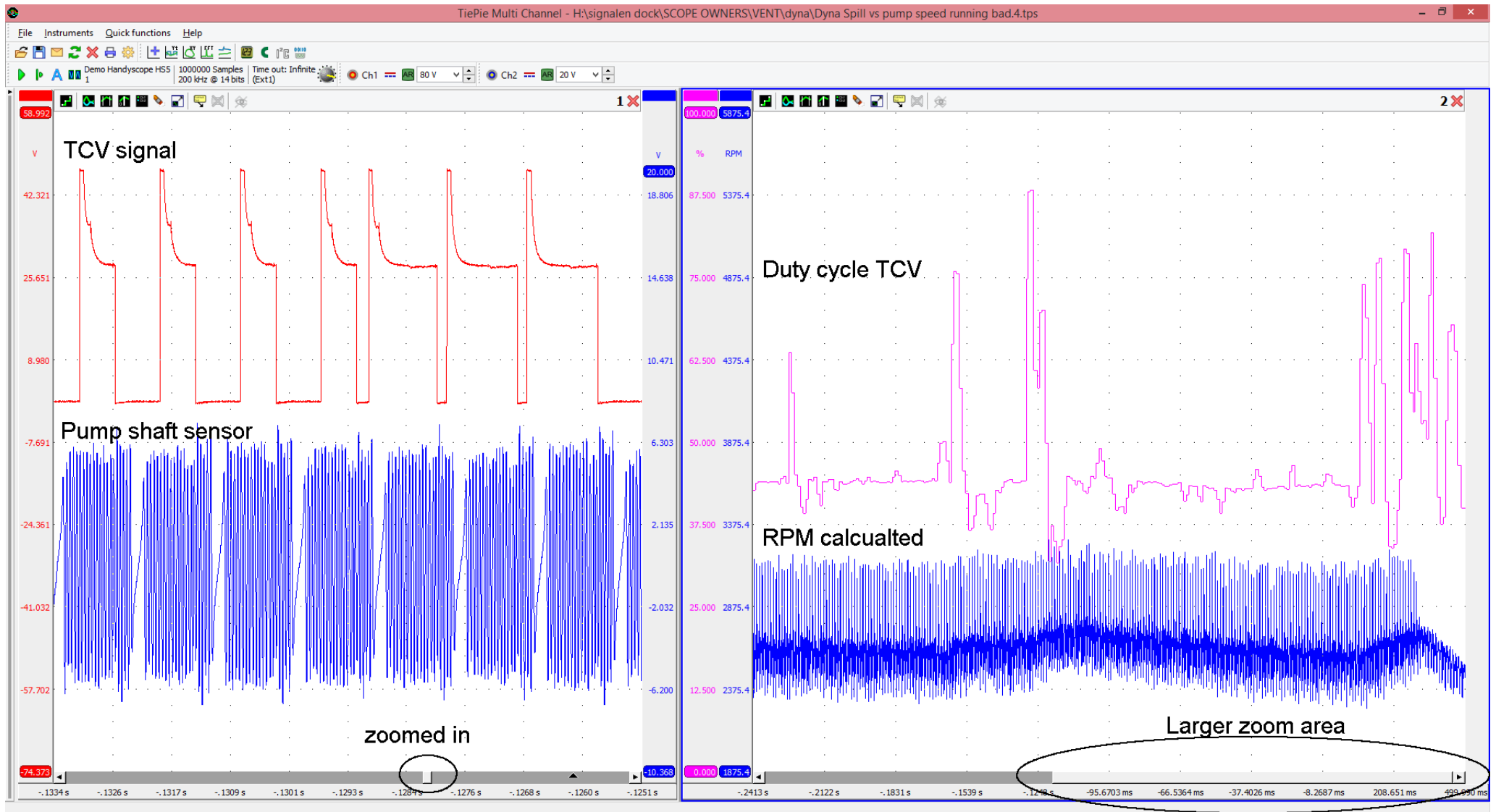
Picture 2: Zoomed in on ATS 500XM scope recording of TCV vs Pump shaft sensor when the engine is misfiring badly.
