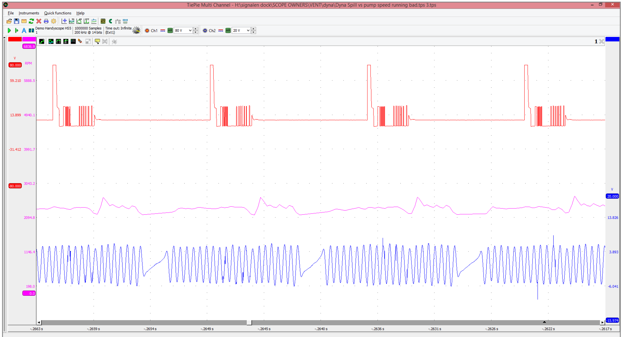
Picture 1: ATS 500XM 2 channel scope recording of Spill valve vs pump shaft sensor
