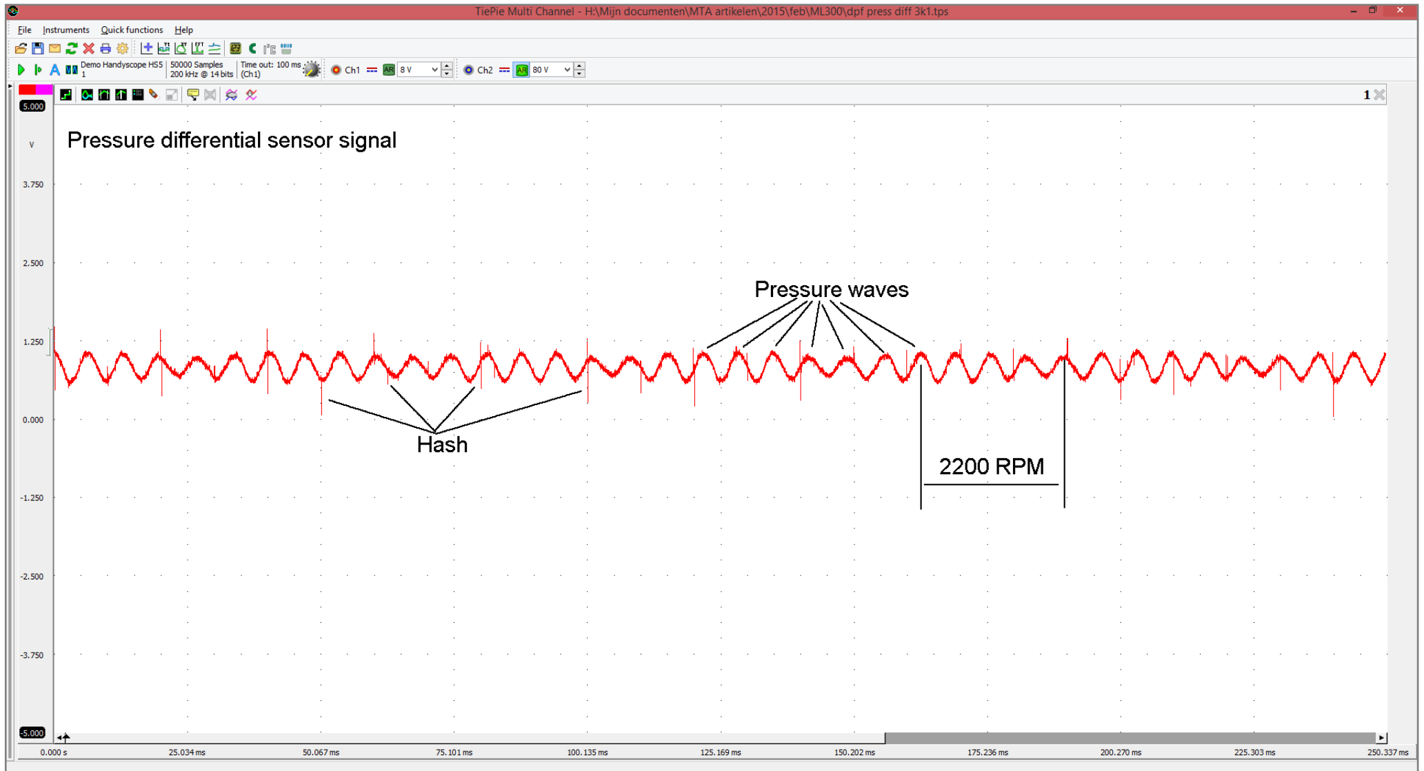
Picture 6: Signal sensor
