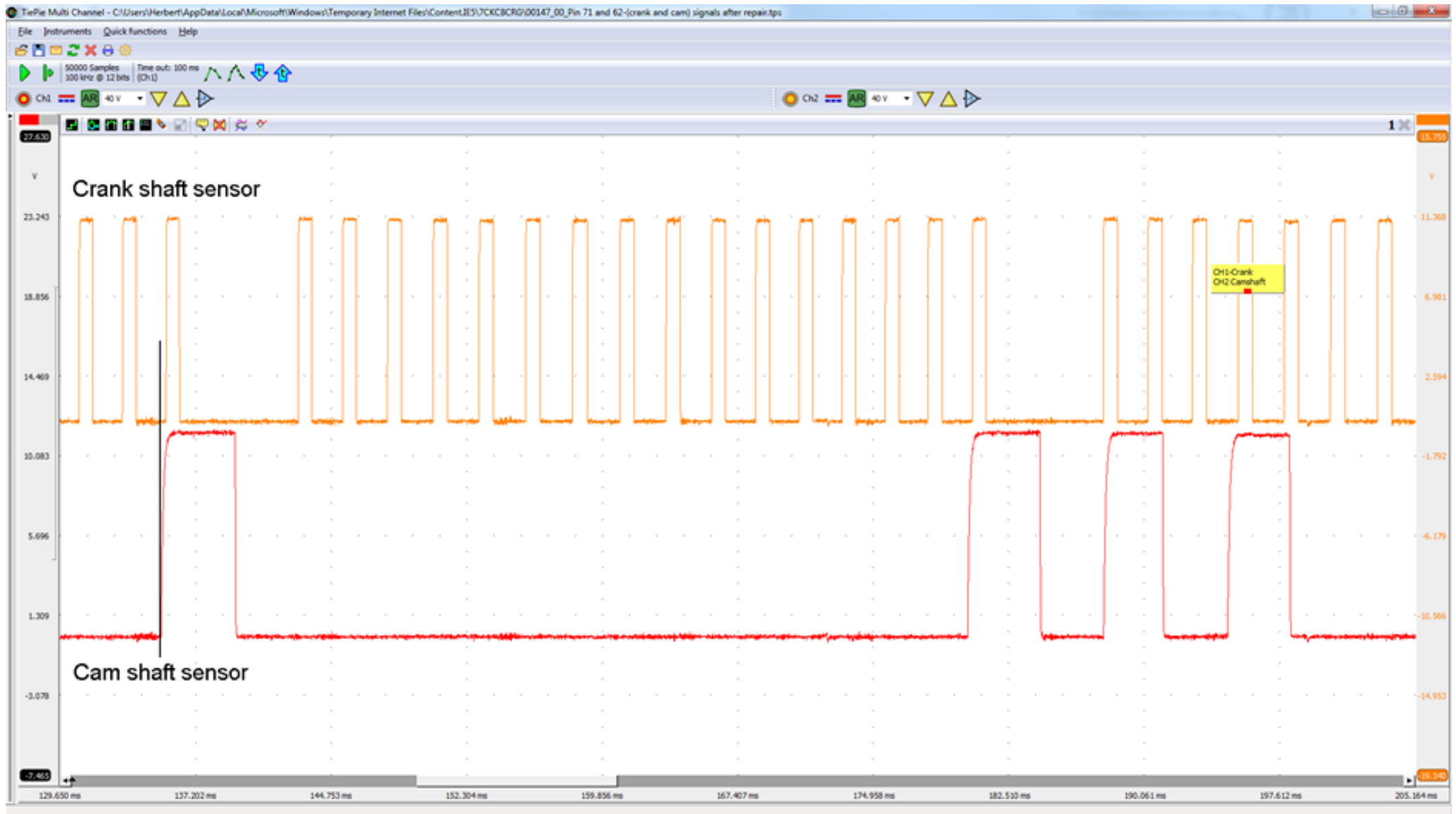
Picture 5 : ATS scope recording of cam vs crank after repair.
