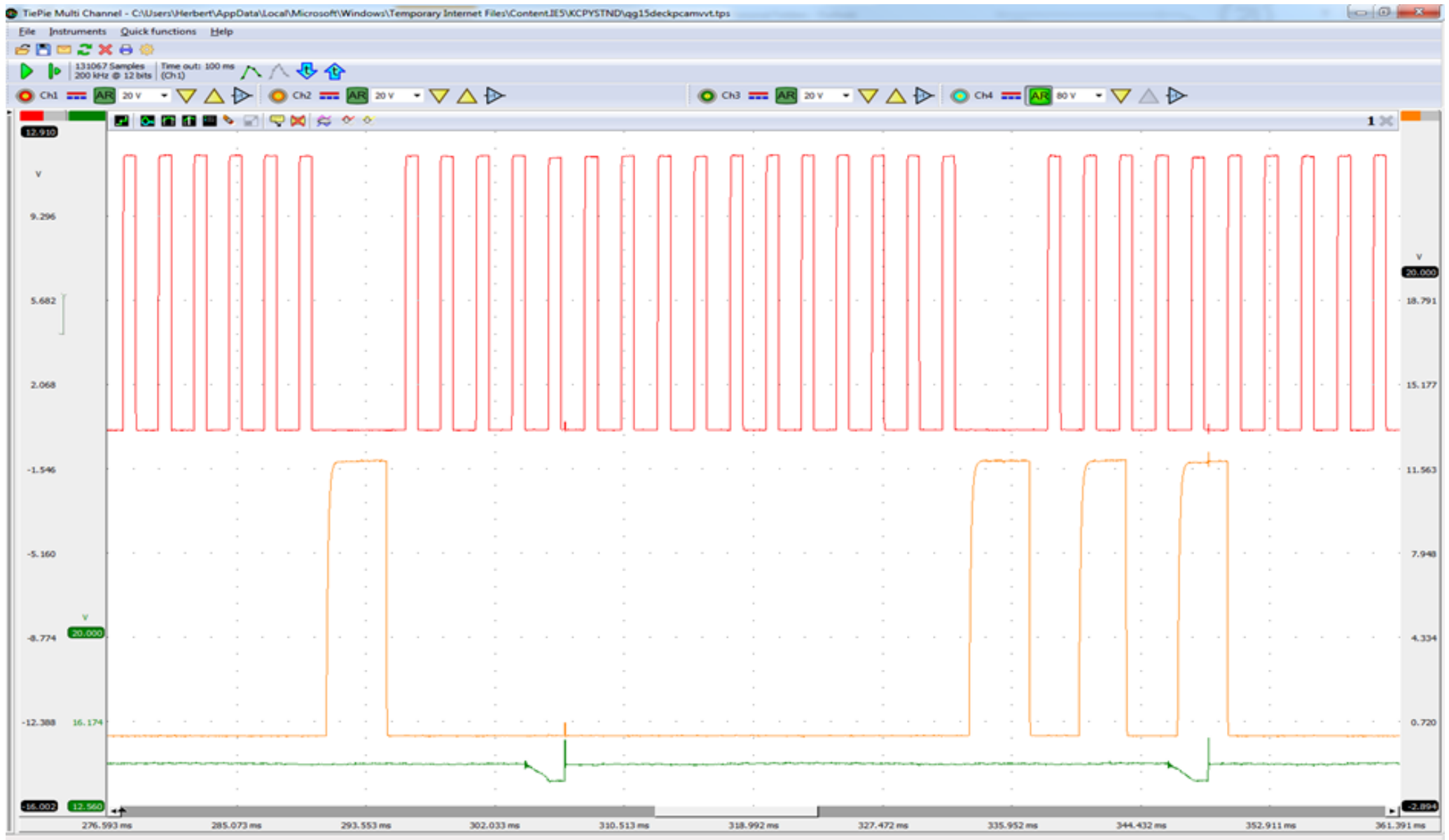
Picture 4 : ATS scope recording on a random good Nissan
