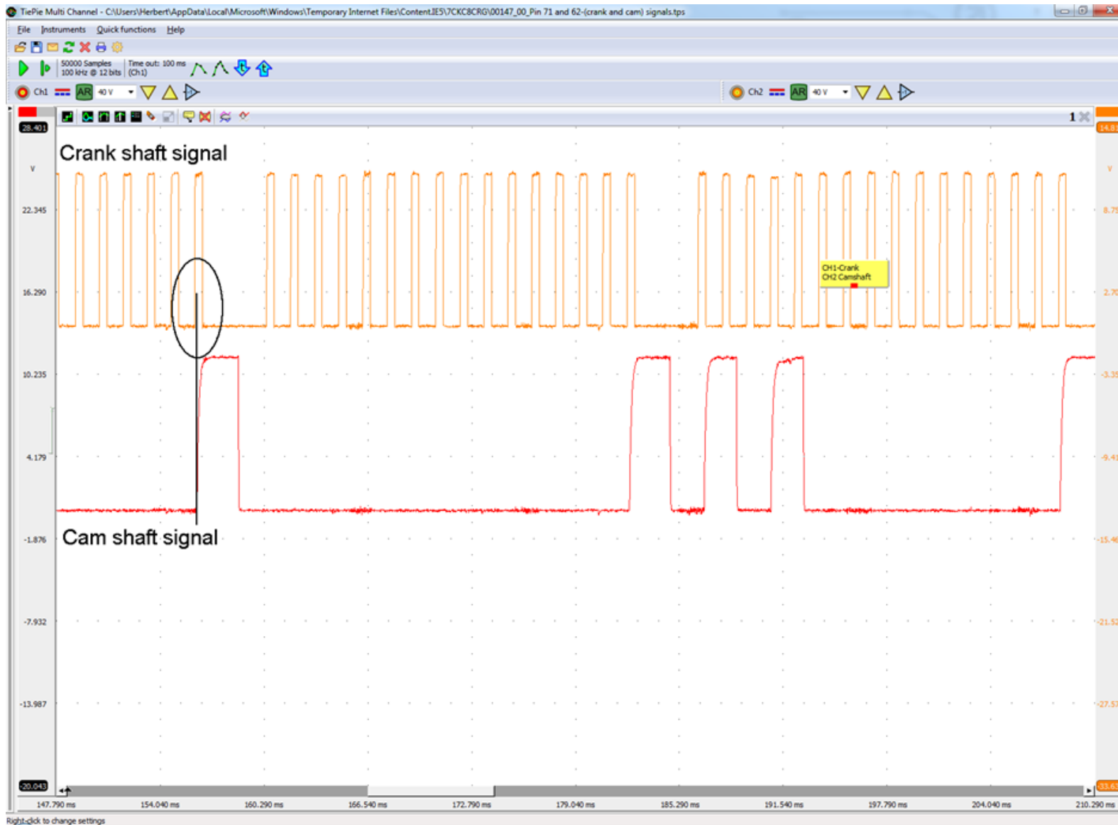
Picture 3 : ATS 5000 scope recording of cam vs crank.
